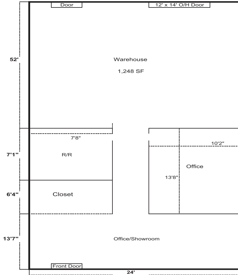
12244 Treeline Ave. Unit 1 Floor Plan
